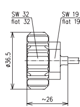
7-16 Stecker 7-16 plug
